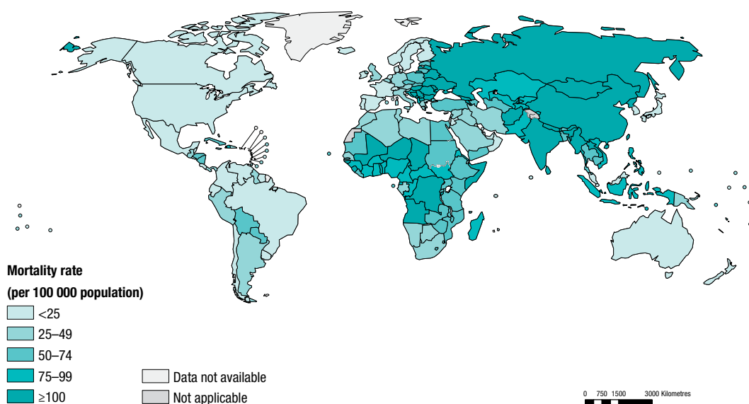
Mortality rate attributed to household and ambient air pollution, by WHO region, 2012 a
